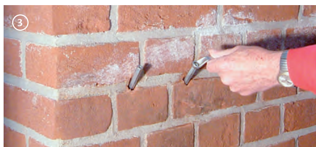
Setting of mechanical packers
