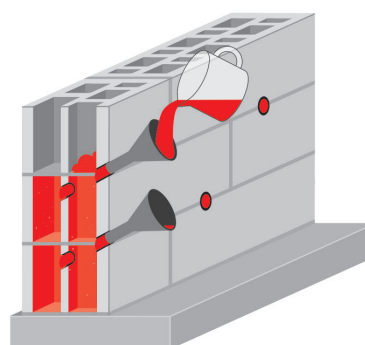
Filling of hollow bricks
