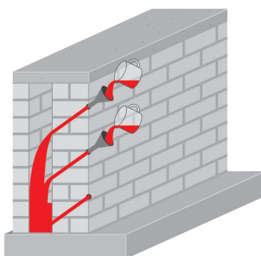
Filling of cavities/voids in masonry
