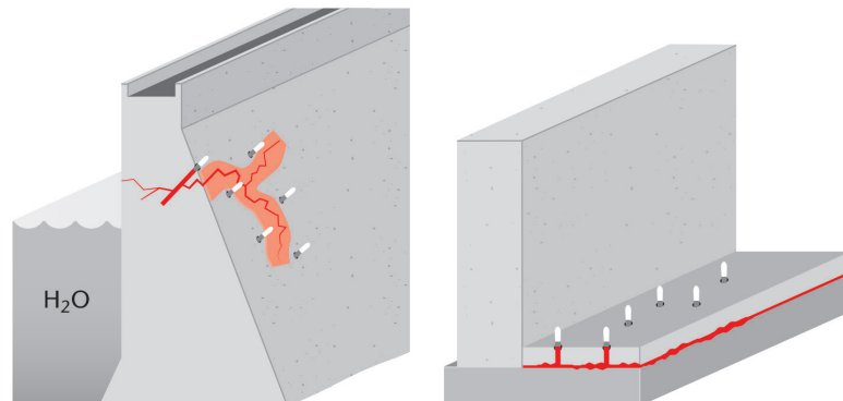
Crack injection in civil engineering structures
