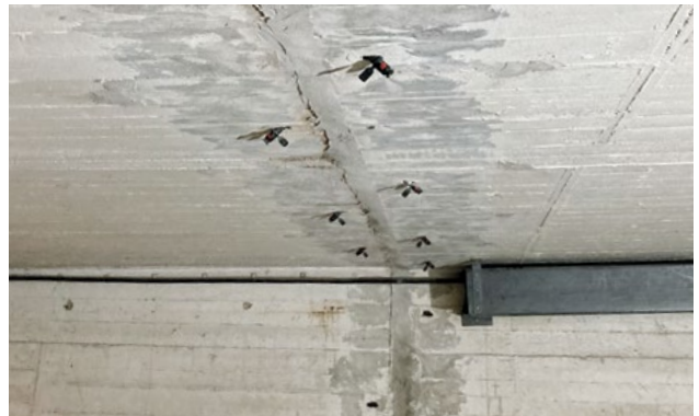
Fig. 4: Patching joint areas, drilling holes and installing packers
